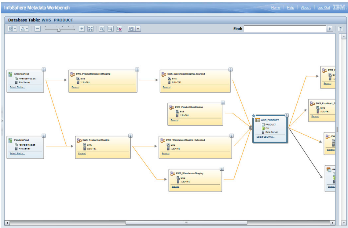
Figure 12-2 View of data lineage
