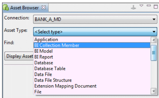
Figure 5-21 Asset Browser
