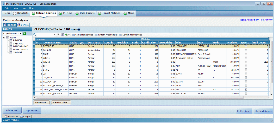
Figure 8-21 Column analysis results
