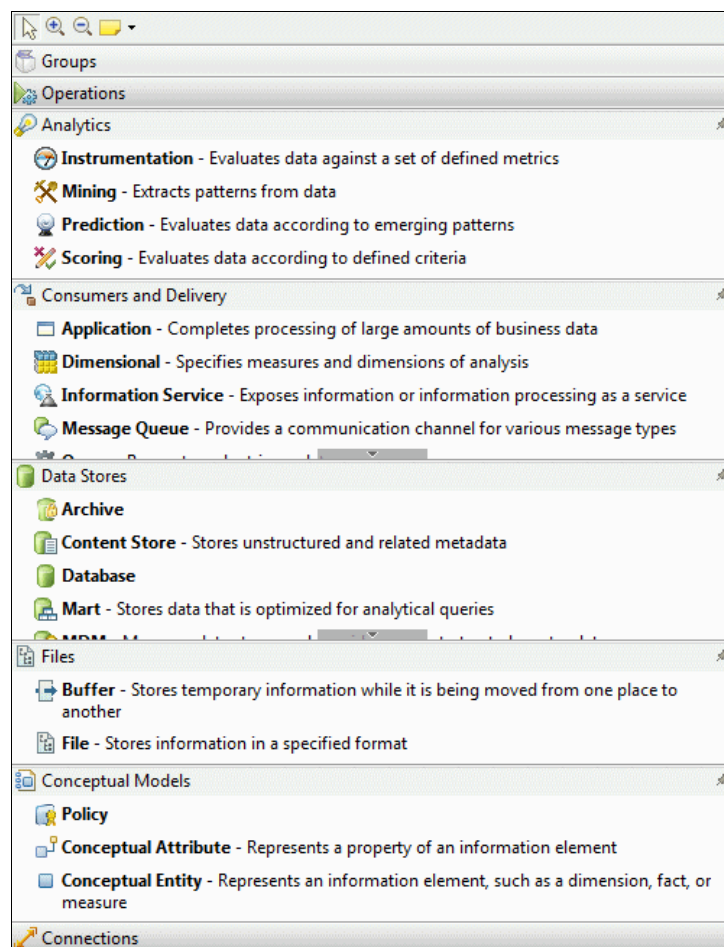
Figure 5-5 Blueprint palette
