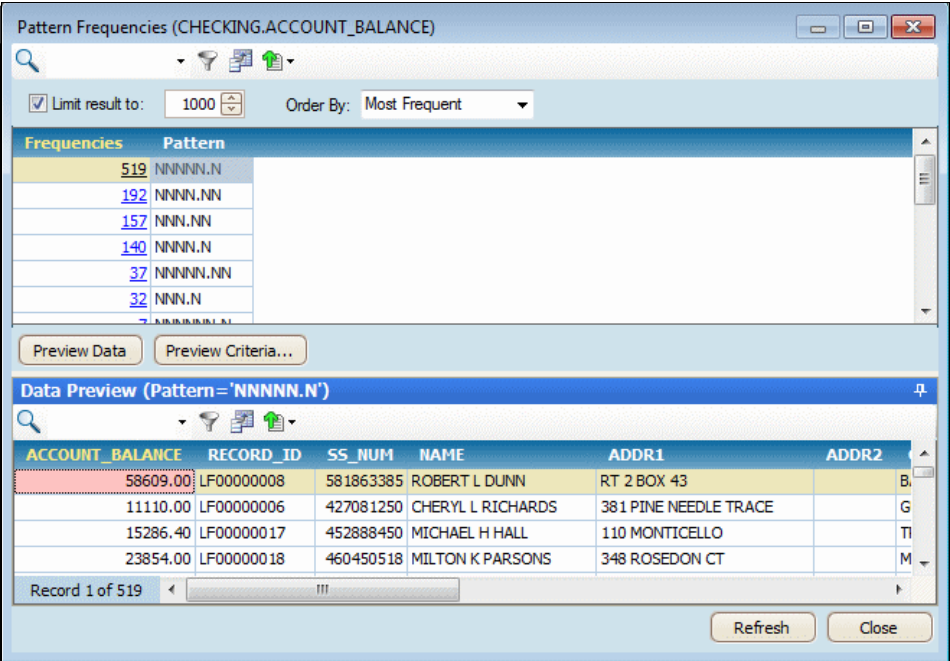
Figure 8-25 Pattern Frequencies
