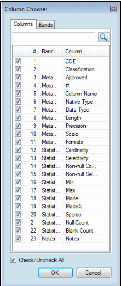
Figure 8-22 Column Chooser
