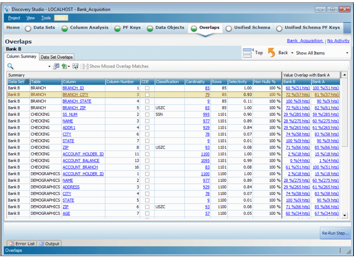
Figure 8-51 Overlaps Column Summary page
