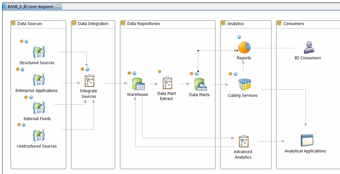
Figure 5-12 Template domains
