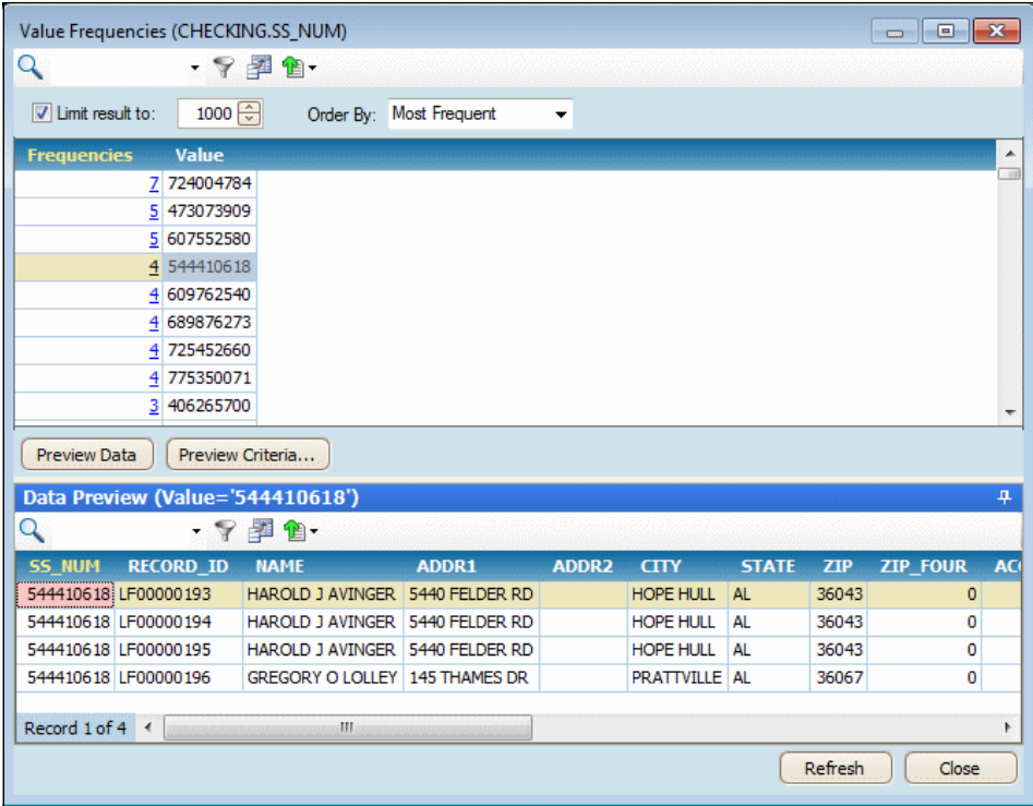
Figure 8-24 Value Frequencies
