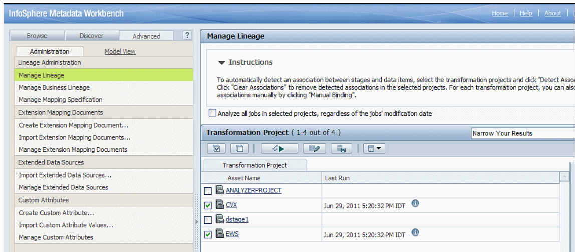
Figure 12-8 Manage Lineage pane
