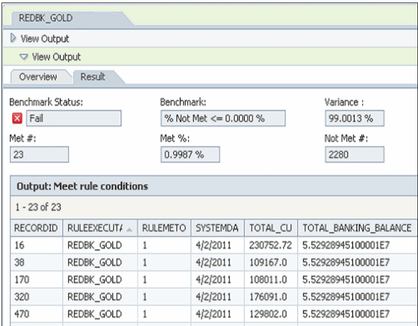
Figure 9-21 Gold customers outputs
