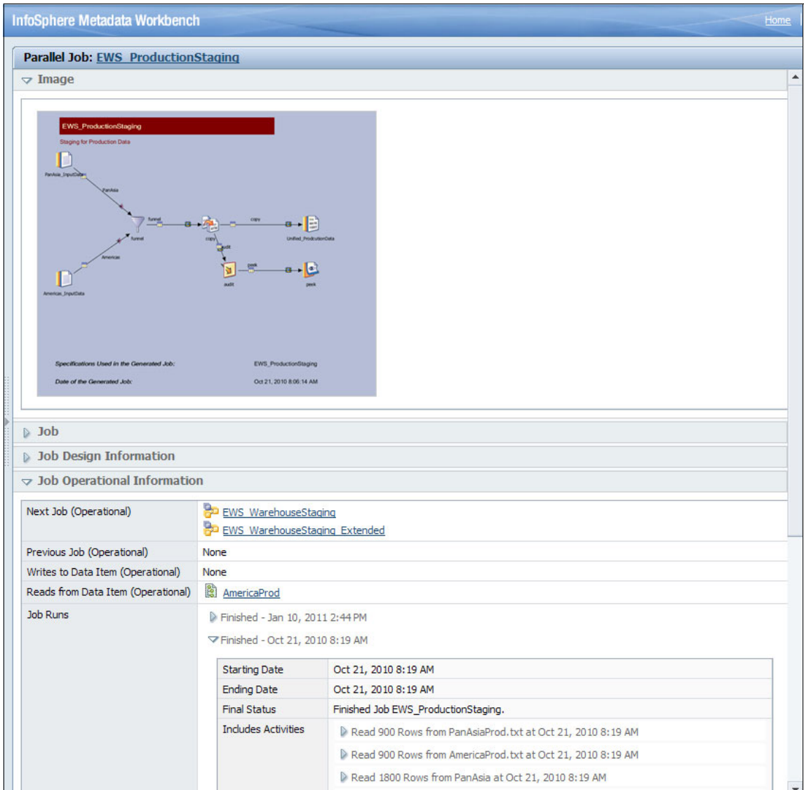
Figure 12-13 Display of InfoSphere DataStage job run information in InfoSphere Metadata Workbench
