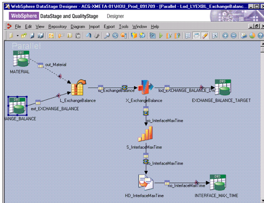
Figure 11-7 InfoSphere DataStage and InfoSphere QualityStage Designer
