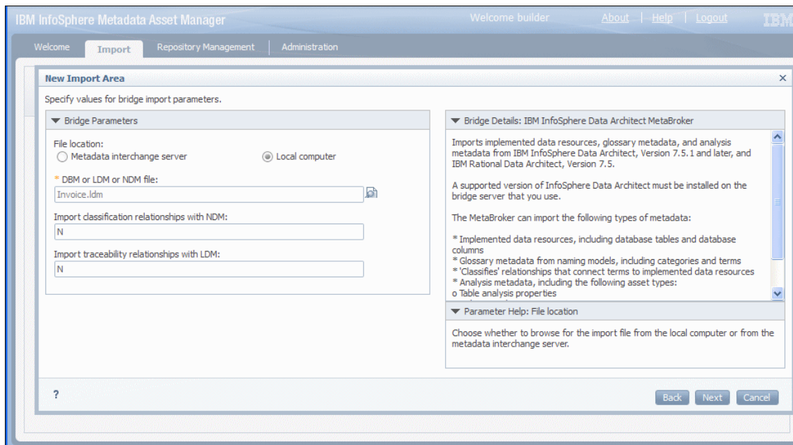
Figure 10-4 Bridge parameters in the import area
