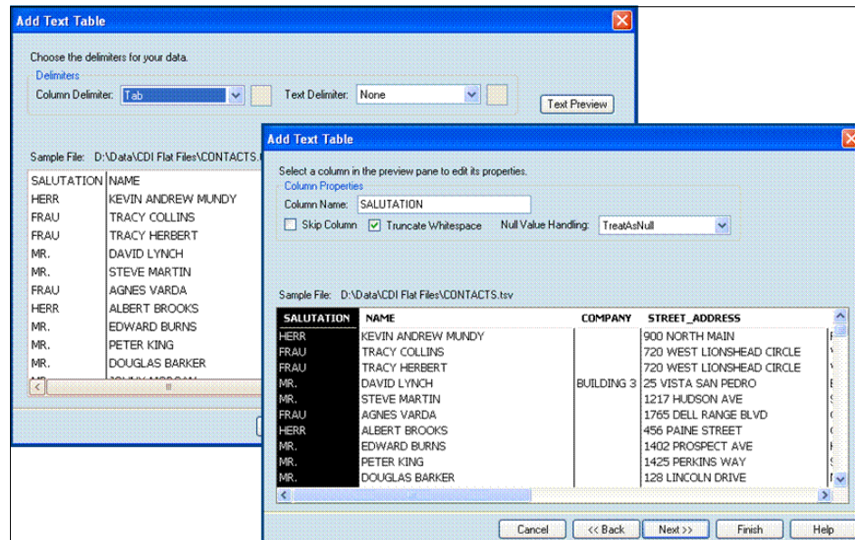
Figure 8-15 Defining the column delimiter and column properties
