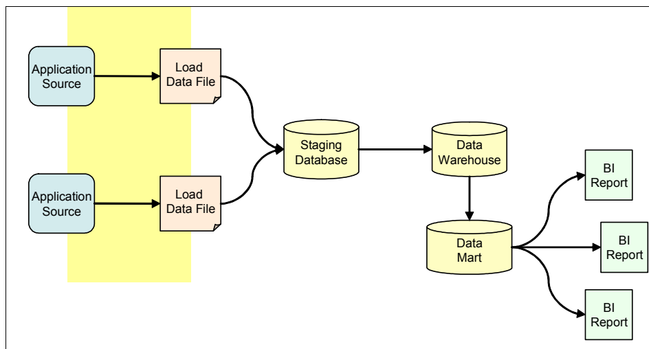
Figure 7-23 Data extraction from data source assets
