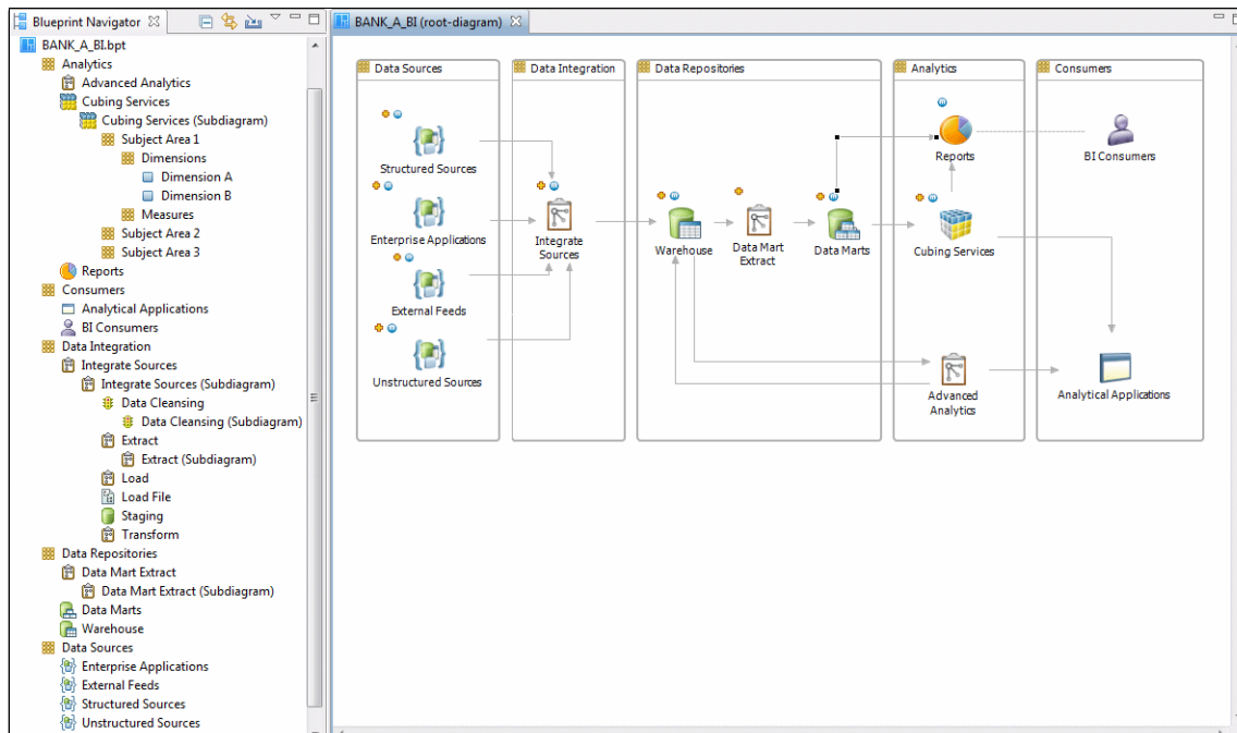
Figure 5-11 Blueprint structure
