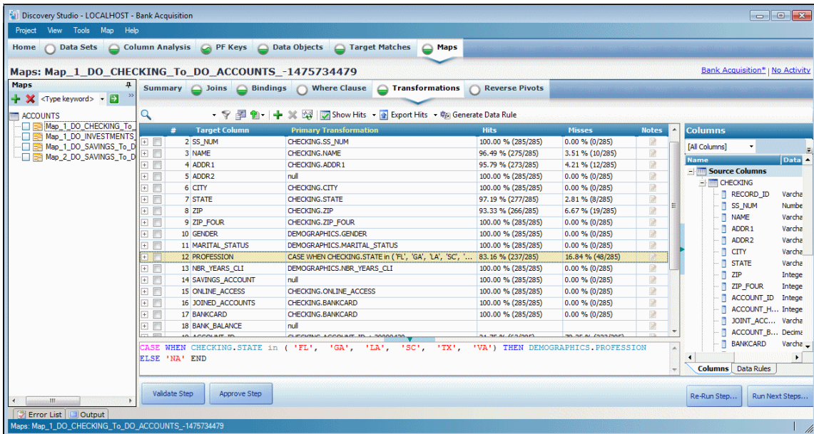
Figure 8-60 Maps Transformations page
