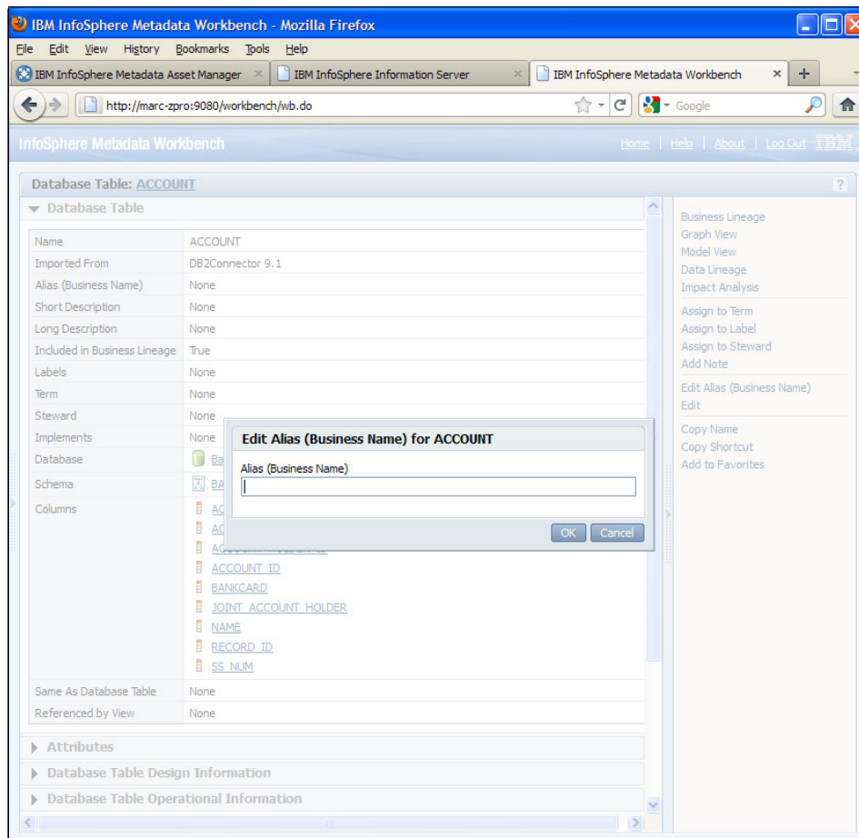
Figure 10-22 Authoring an alias name for a database table
