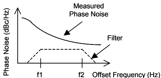
Figure 10. Phase Jitter is calculated by applying an industry-defined filter to a phase-noise graph and integrating across frequency to calculate an RMS number.
