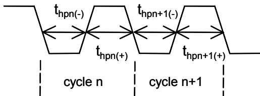
Figure 9. Waveform for HP-C2C Jitter Calculation
