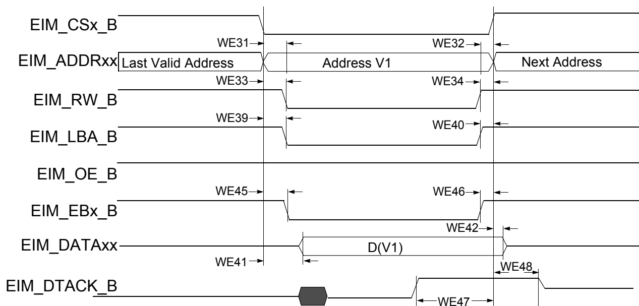
Figure 21. DTACK Write Access (DAP=0)
