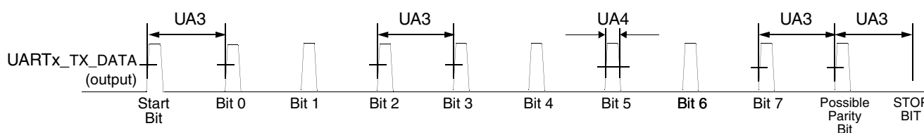
Figure 51. UART IrDA Mode Transmit Timing Diagram
