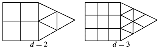
Figure 8: Each face is divided in d \times d smaller one.
