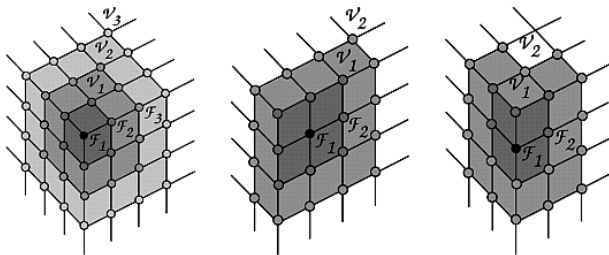
Figure 9: Vertex [face] neighborhoods \mathcal{V}_k [ \mathcal{F}_k ] are defined by adding one more ring to the previous set.
